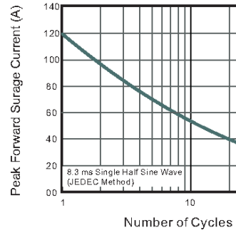
Fig.6 Maximum Non-Repetitive Peak Forward Surge Current
