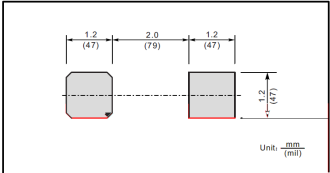
The recommended mounting pad size
