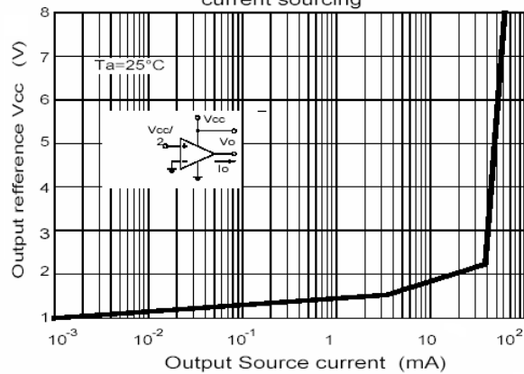
Fig.9 Output Characteristics current sourcing T_a=25^{\circ}C
