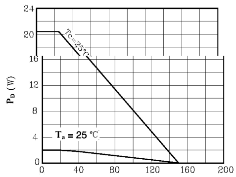
P_D - T_a
