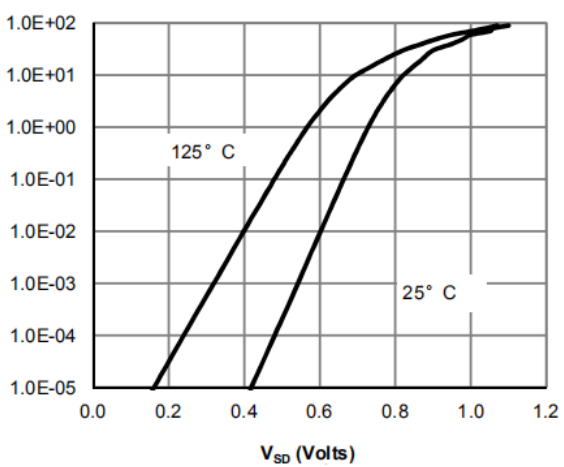
Figure 6: Body-Diode Characteristics
