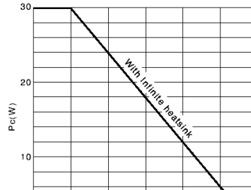
Reverse Bias Safe Operating Area
